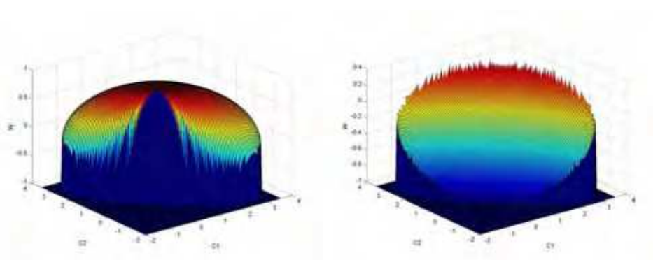
Figure 3 Relationship between lower(left) and higher(right) range of \omega and c_1, c_2 to guarantee the convergence of iterative process \{DX_t\}
