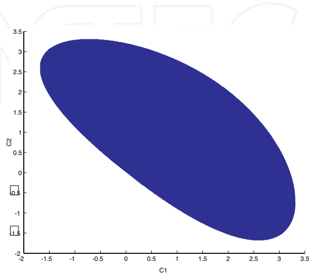
Figure 2 Relationship between c_1 and c_2 to guarantee the convergence of iterative process \{DX_t\}
